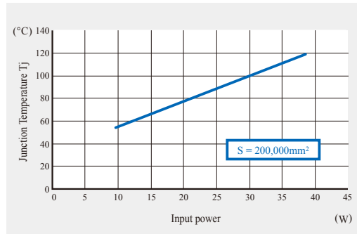
Figure3 (b)-6 Input power - junction temperature Tj (CLU034-1206B8)
