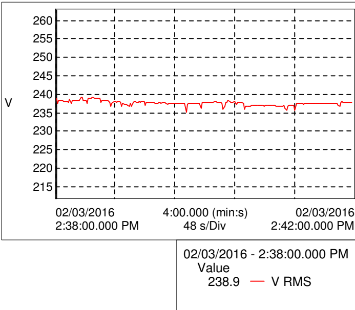
Graph - Voltage(Vrms)
