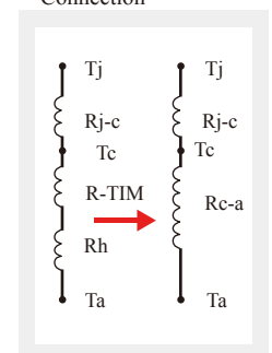
■Figure-1 ( b ) Thermal Resistance Connection
