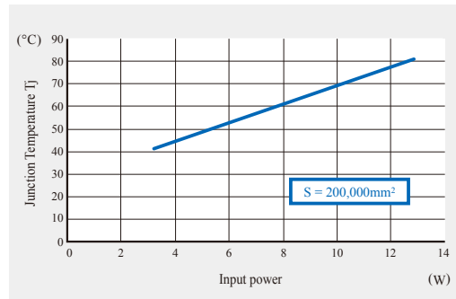
Figure3 (b)-2 Input power - junction temperature Tj (CLU024-1202B8)
